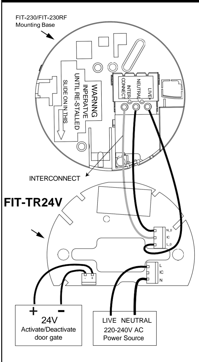
Fig.1. Installation Instruction (connect with 1 pcs smoke alarm)
