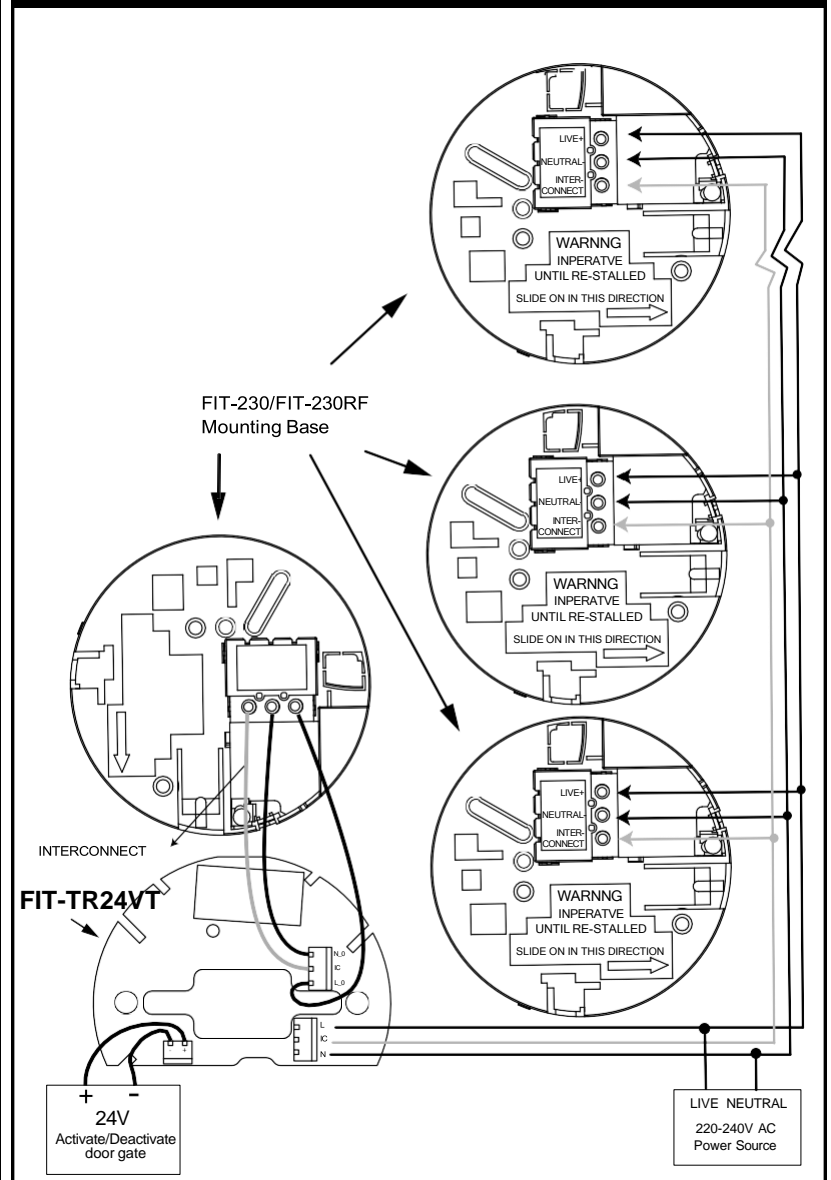
Fig.2. Installation instruction (more than 1 pcs smoke alarm)
